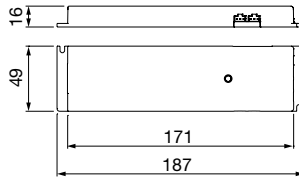
X-Driver 15 W
