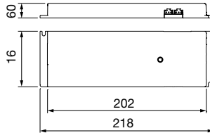
X-Driver 30 W
